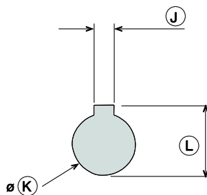
DRIVEN SHAFT SECTION (BARE SHAFT)
